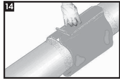
Centre the closure on the overlapping sleeve. Press down firmly.
