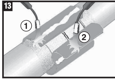
Wrap the sleeve loosely around the pipe, ensuring the appropriate overlap. Gently heat the backing of the underlap and the adhesive side of the overlap. Press the overlap into place.
